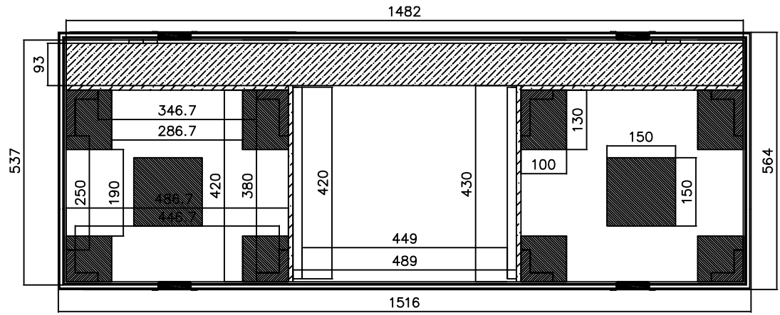
Top View Base
